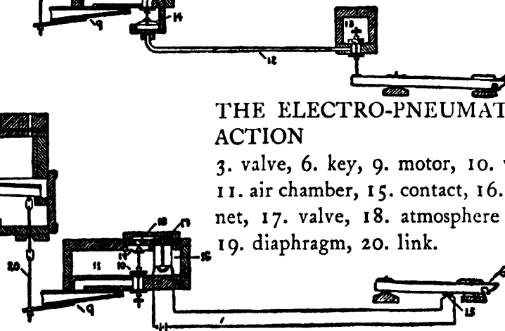
FIGURE 159. Evolution of the action.
